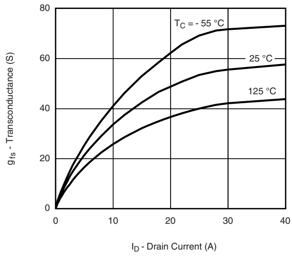
Transconductance
