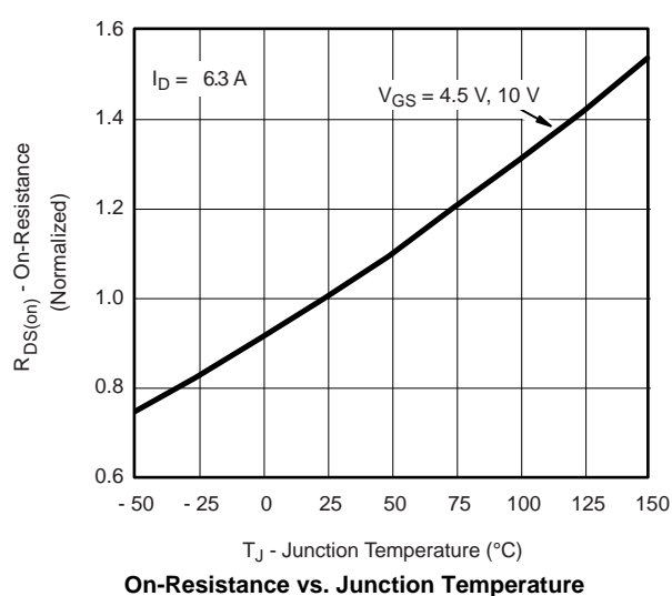
T_J - Junction Temperature ( ^\circ\text{C} ) On-Resistance vs. Junction Temperature
