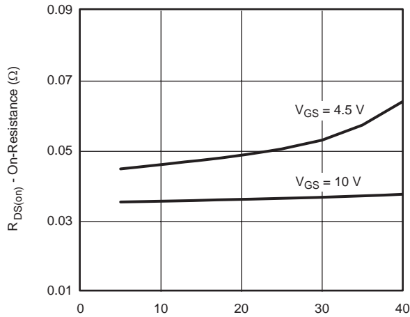
V_{GS} = 4.5\text{ V} V_{GS} = 10\text{ V} On-Resistance vs. Drain Current
