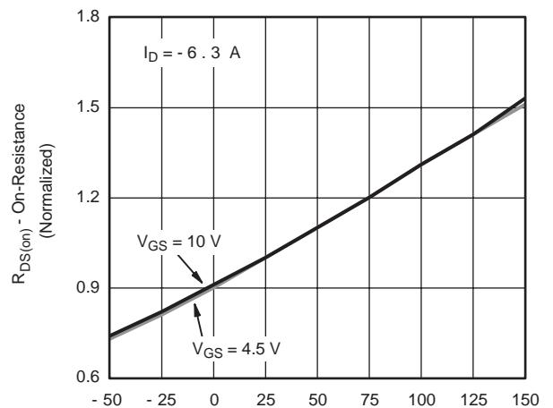
I_D = 6.3\text{ A} V_{GS} = 10\text{ V} V_{GS} = 4.5\text{ V} On-Resistance vs. Junction Temperature
