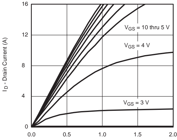
V_{GS} = 10 thru 5 V V_{GS} = 4 V V_{GS} = 3 V Output Characteristics
