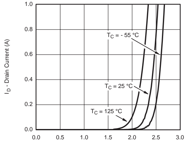
T_C = -55^\circ\text{C} T_C = 25^\circ\text{C} T_C = 125^\circ\text{C} Transfer Characteristics
