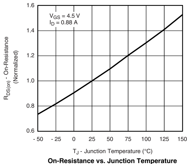
T_J - Junction Temperature ( ^\circ C ) On-Resistance vs. Junction Temperature
